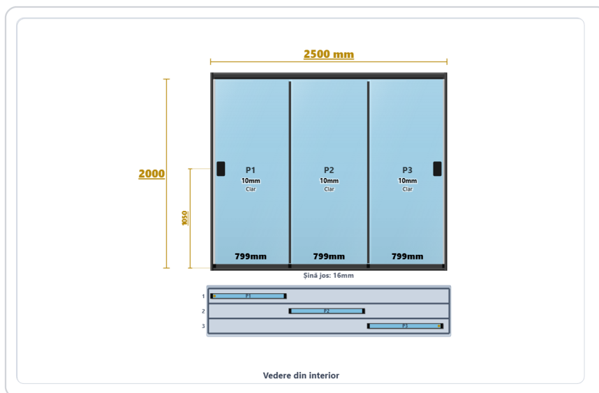
2500 x 2000 mm | 3 panouri | Sticla 10mm Clar
